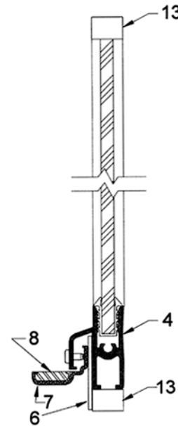
ELEVATION VIEW
